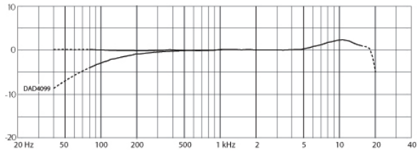
Typical on- and off-axis frequency response of DPA 4099 with DAD4099 XLR adapter at 20 cm (7.9 in) distance
